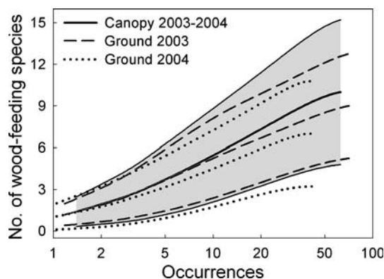
Fig. 4 Rarefaction curves for assemblages of wood-feeding termites from canopy sampling (pooled 2003–2004 campaigns: solid lines, shaded area) compared with ground sampling campaigns (dashed and dotted lines). Graphs show averages and 95% confidence intervals, calculated by the Mao-Tau method (Colwell et al. 2004). Abscissa is scaled logarithmically
