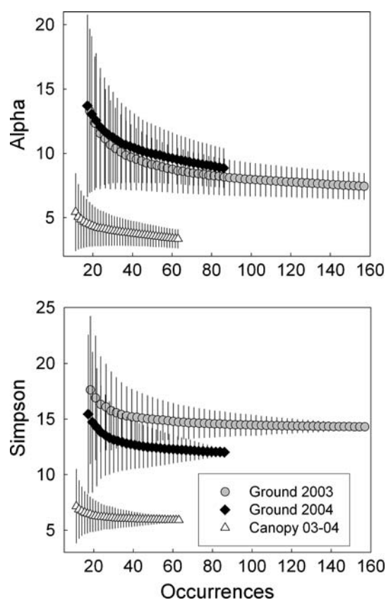
Fig. 3 Fisher's alpha ( top ) and Simpson's inverse index ( 1/D ) ( bottom ) for ground and canopy samples (mean \pm standard deviation)
