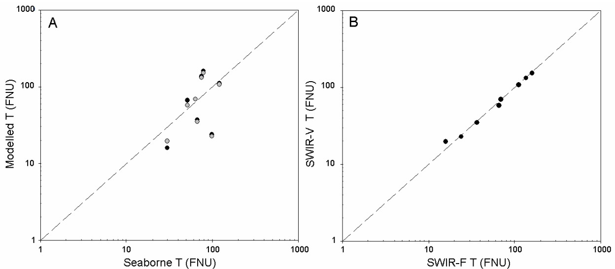
Figure 8. A) Scatter plot of seaborne and modelled turbidity (T) using the SWIR-V (grey) and SWIR-F (black) atmospheric correction approaches for stations with T_{ind} > 1.3 ; B) Comparison of MODIS-derived T from the two approaches.
